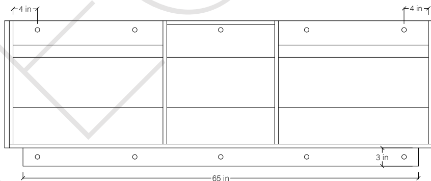
INSIDE BACK VIEW
