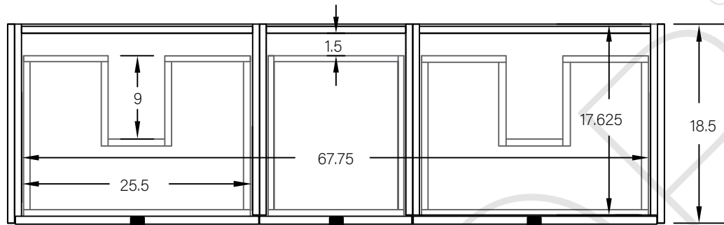
TOP VIEW
