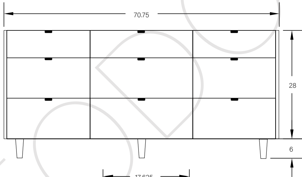
FRONT VIEW
