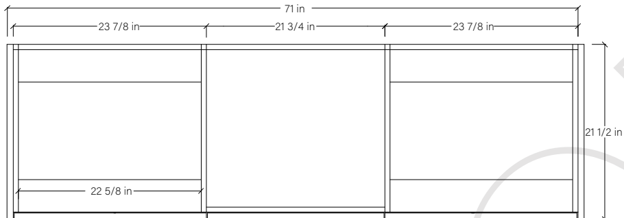
TOP VIEW
